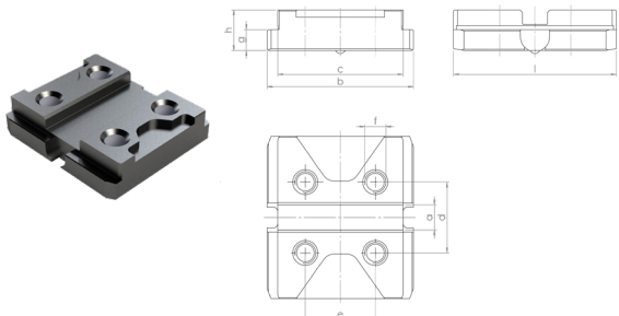
Jaw adapter for CentroGripp/T-Rex
